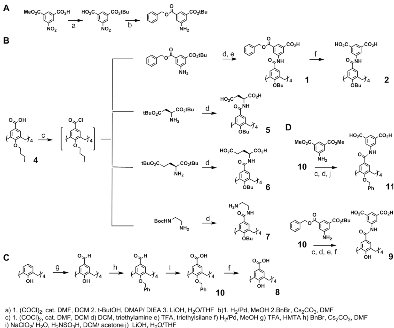
Figure 1. Synthetic routes for: (A) upper rim modifications, mono- t -butyl-5-aminoisophthalate. (B) Lower rim n -butyl modifications on compounds 1 , 2 and 4 – 7 . (C) Lower rim benzylated compound 10 and tetrahydroxy calix[4]arene 8 . D. Compounds 9 and 11 .
